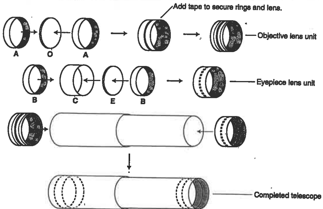
Figure 3. Telescope Construction
